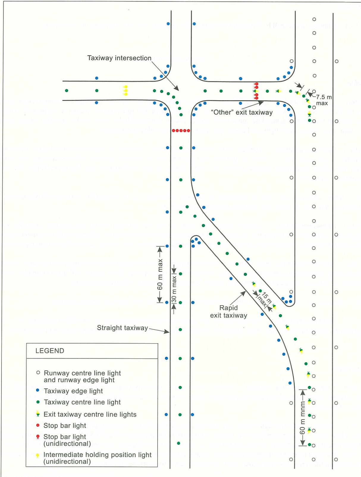
Figure 5-25. Taxiway lighting
