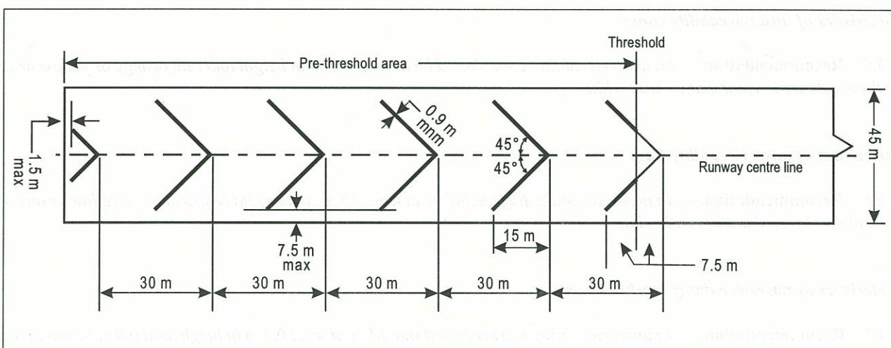
Figure 7-2. Pre-threshold marking
