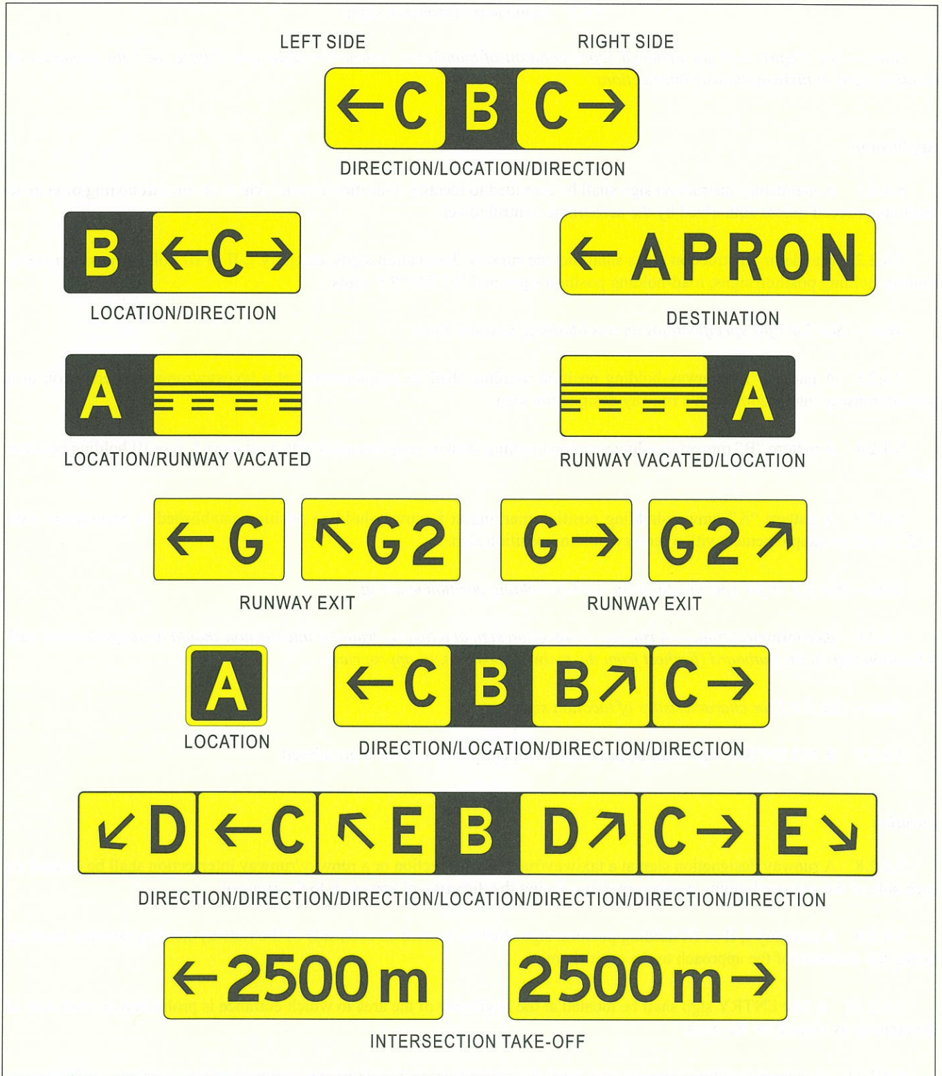
Figure 5-30. Information signs
