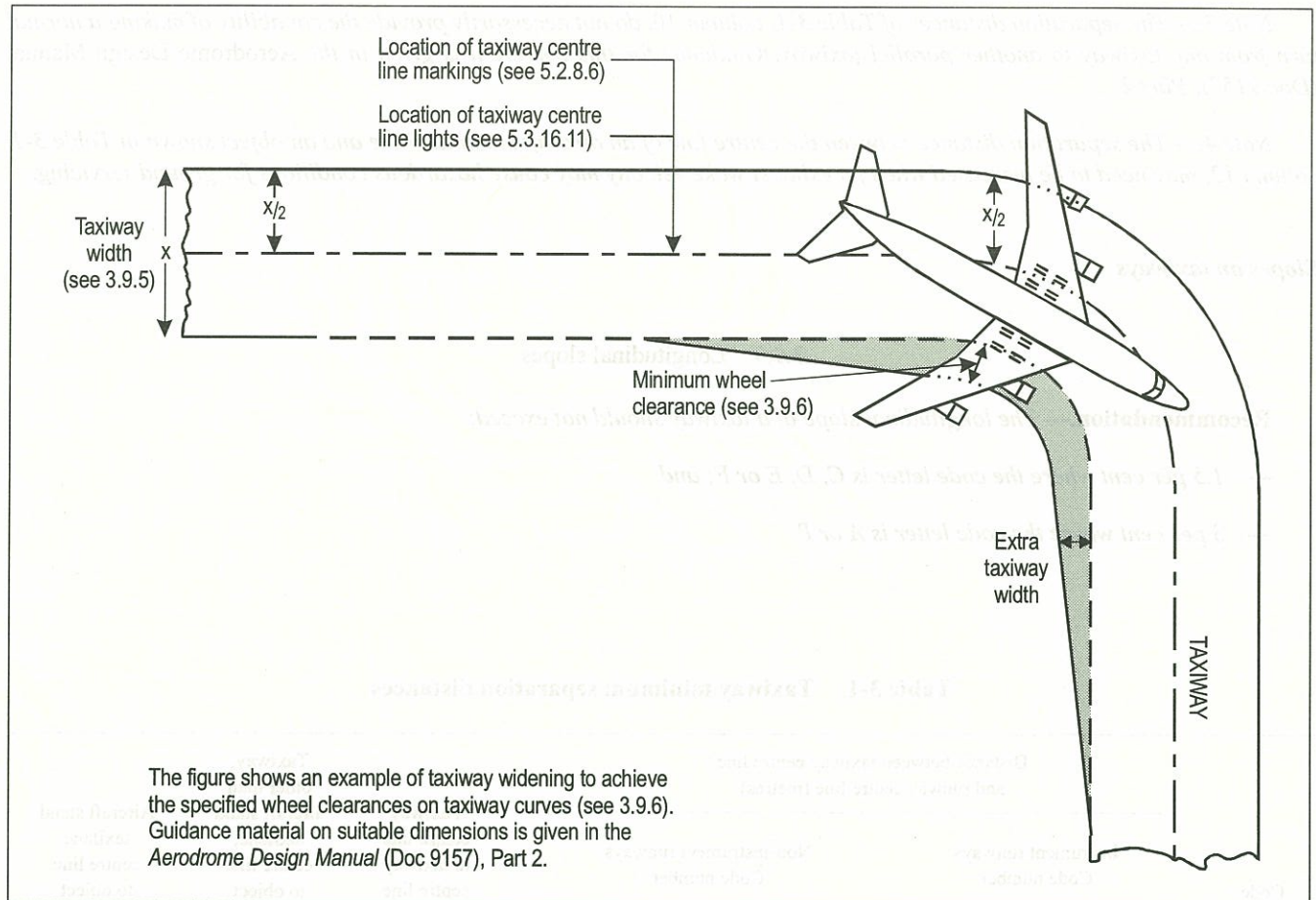
Figure 3-2. Taxiway curve
